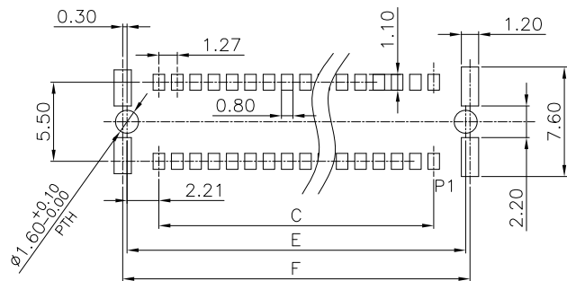
P.C. Board Layout ( TOP View ) (Tolerance \pm 0.05 )
