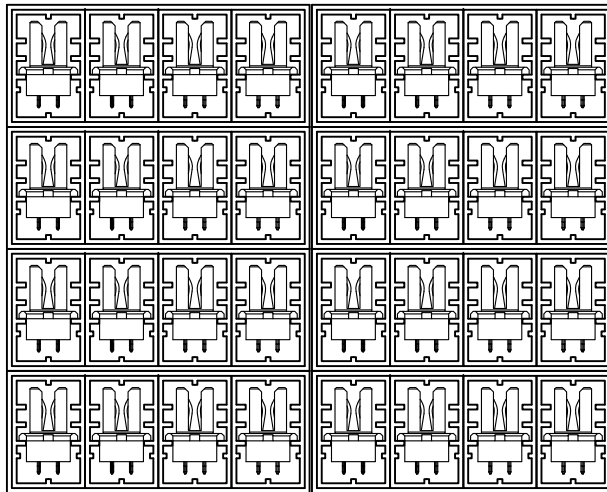
Drawing Three:Lay 2 bundles in each layer.Install in 4 layers.8bundles,32 tubes in all.
