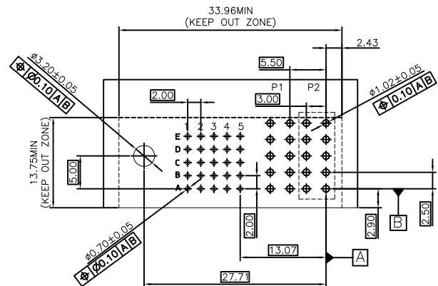
P.C.Board Layout (Tolerance:±0.05)
