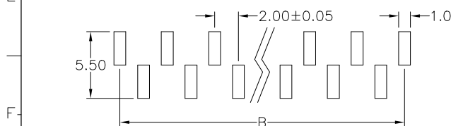
P.C. Board Layout Type A
