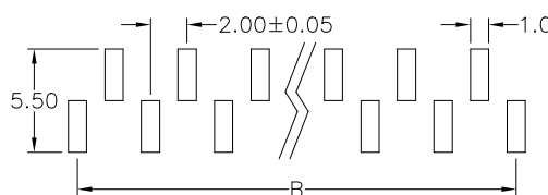
P.C. Board Layout Type B
